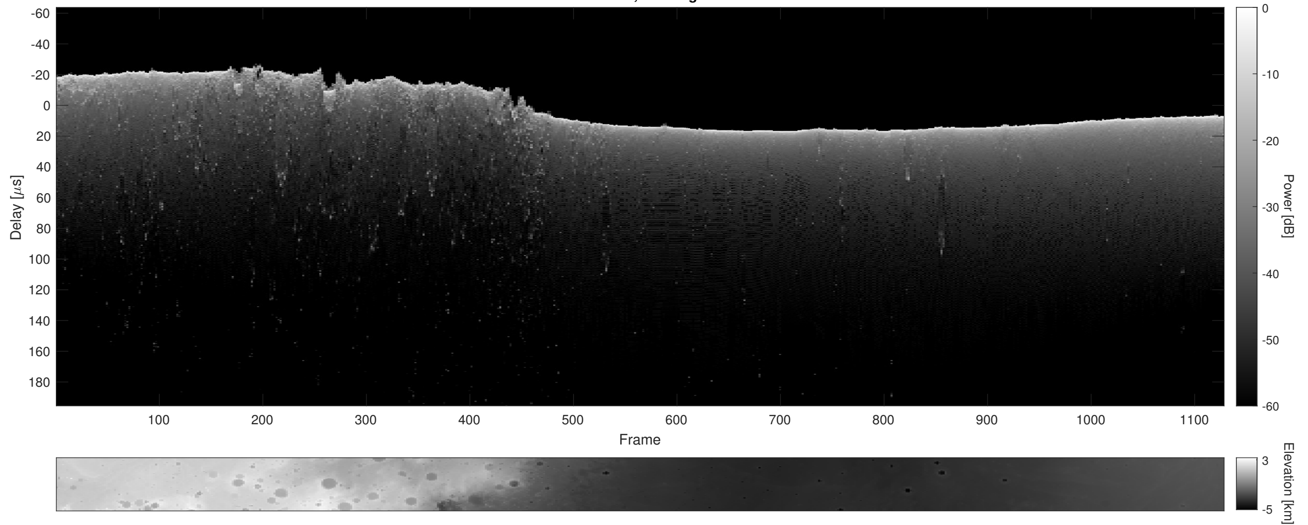
Orbit 14387, Cluttergram
