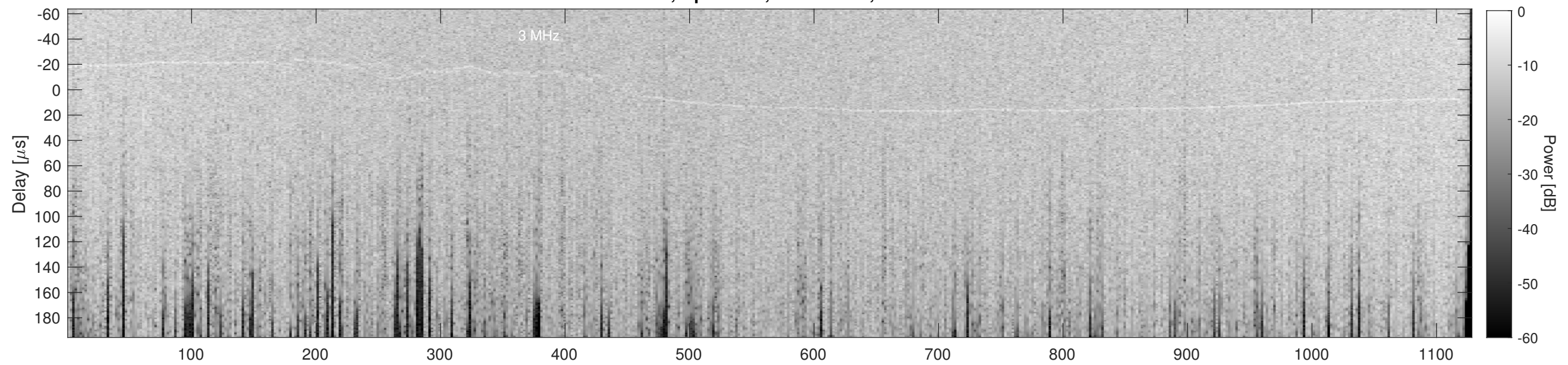
Orbit 14387, Cluttergram
