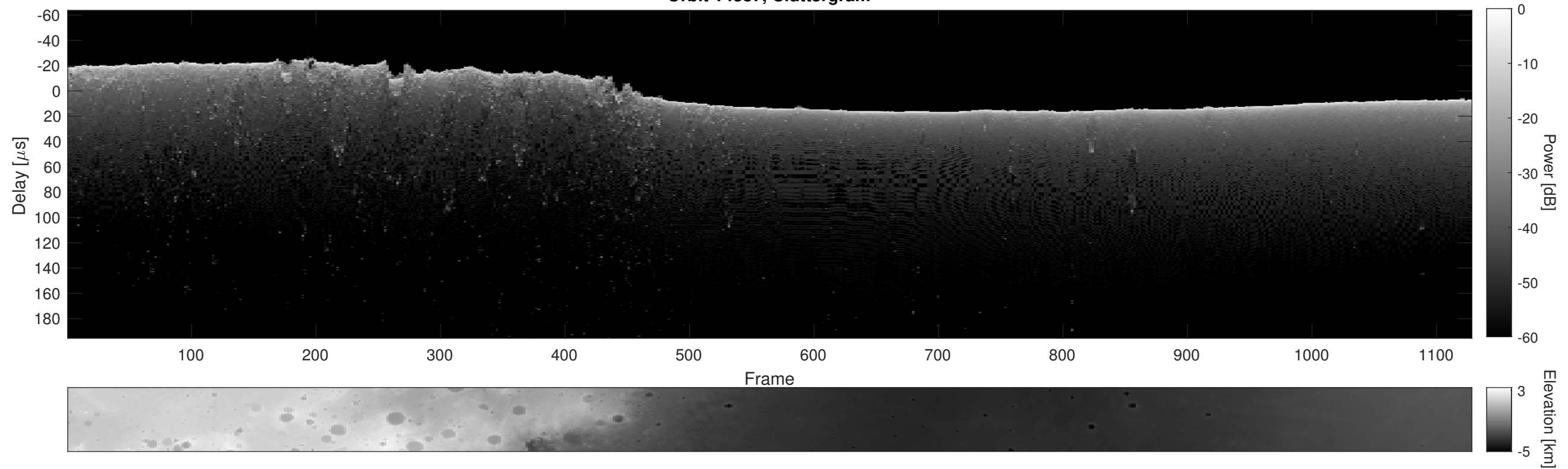
Orbit 14387, Cluttergram
