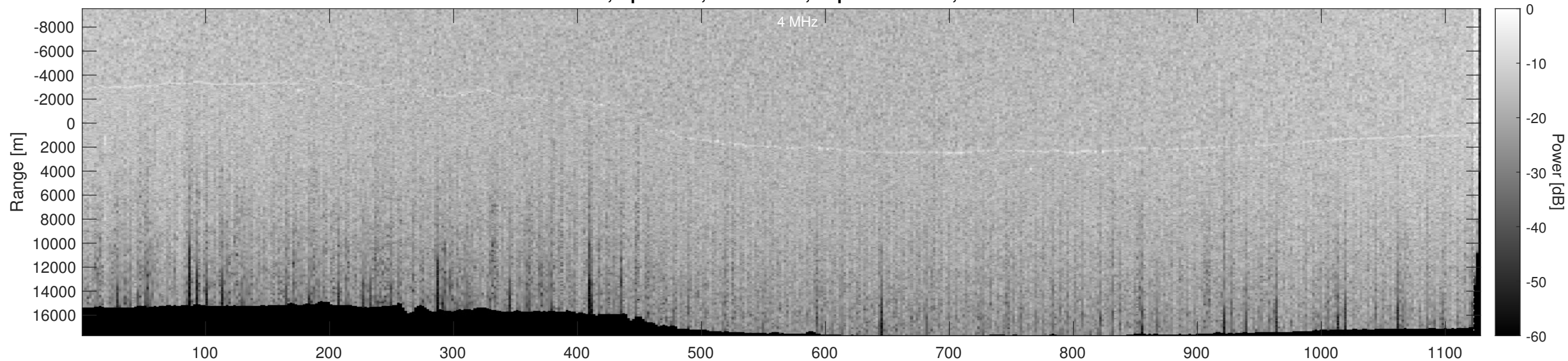
Orbit 14387, Optimized, No Window, Depth-Corrected, Channel 2
