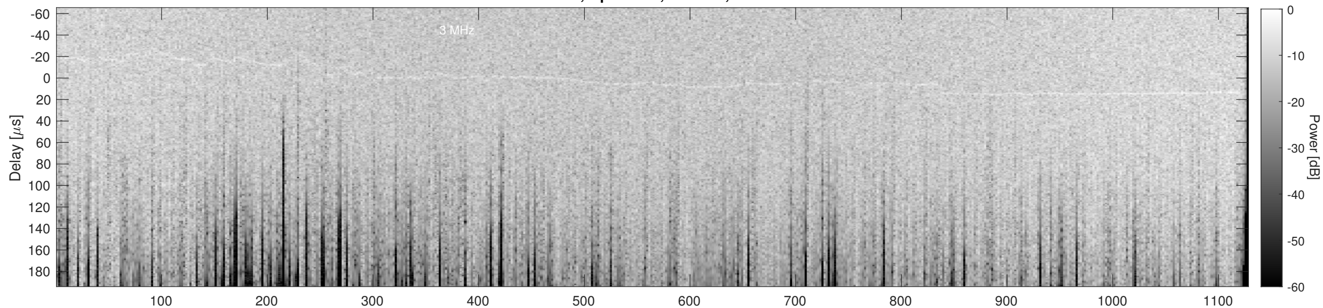
Orbit 14388, Cluttergram
