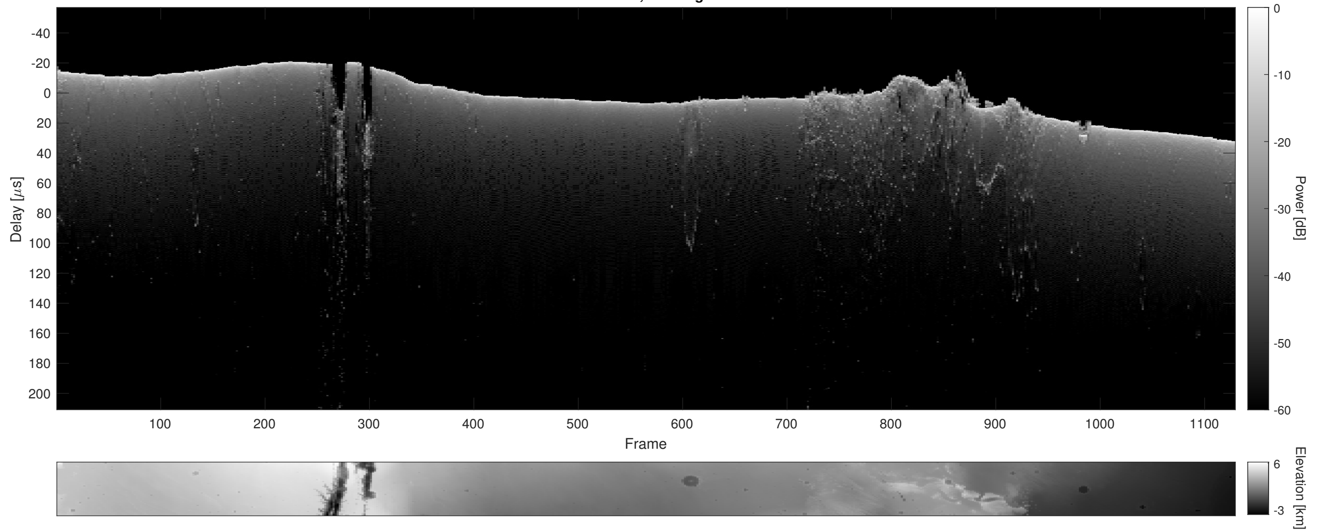
Orbit 14389, Cluttergram
