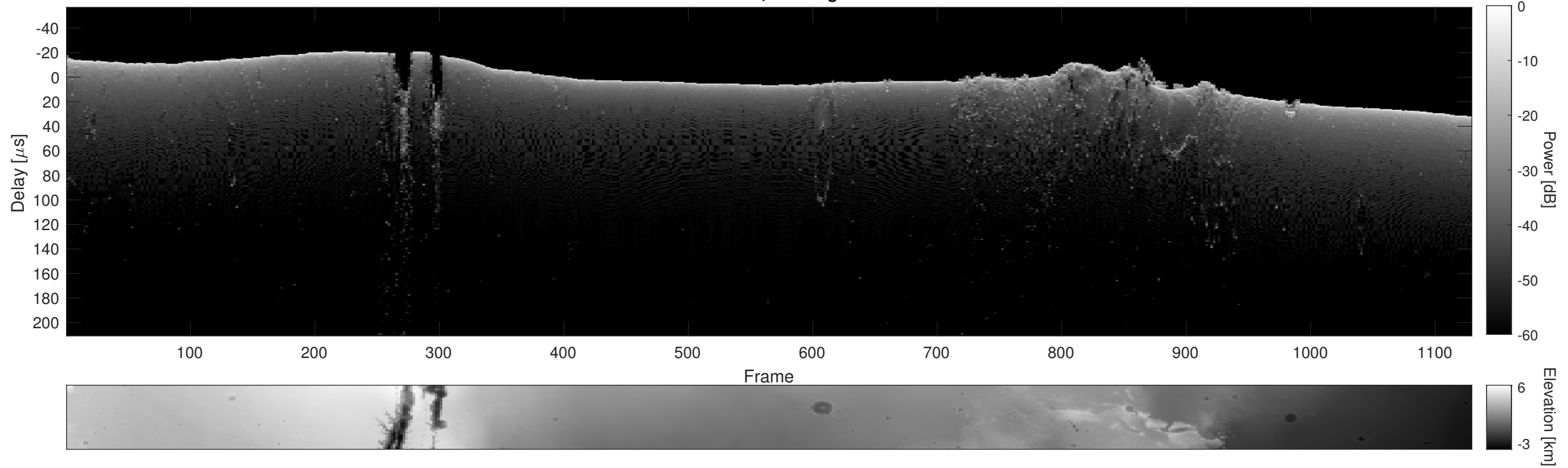
Orbit 14389, Cluttergram
