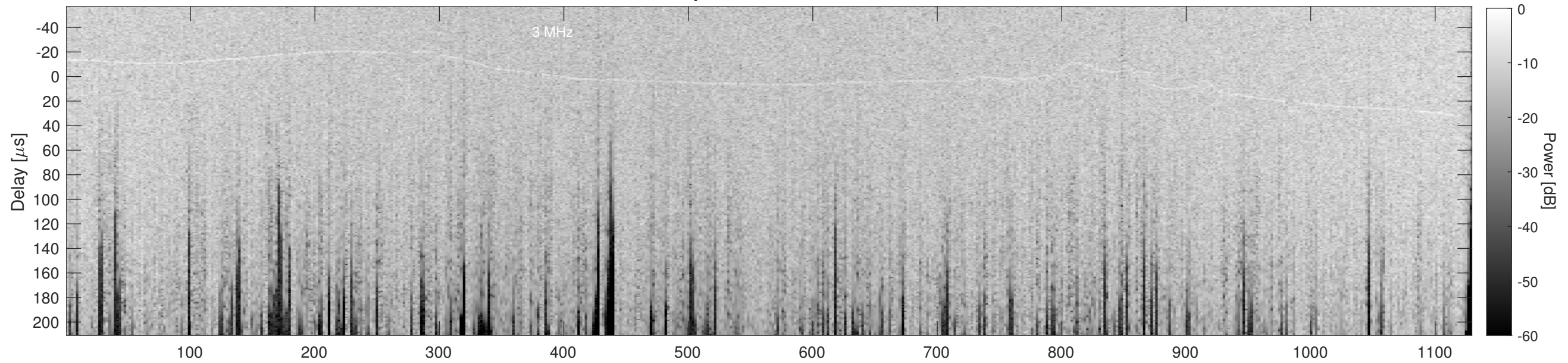
Orbit 14389, Cluttergram
