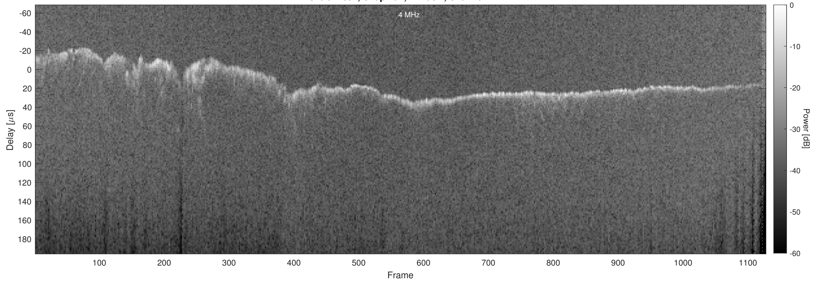
Orbit 14394, Chapman, Window, Channel 2
