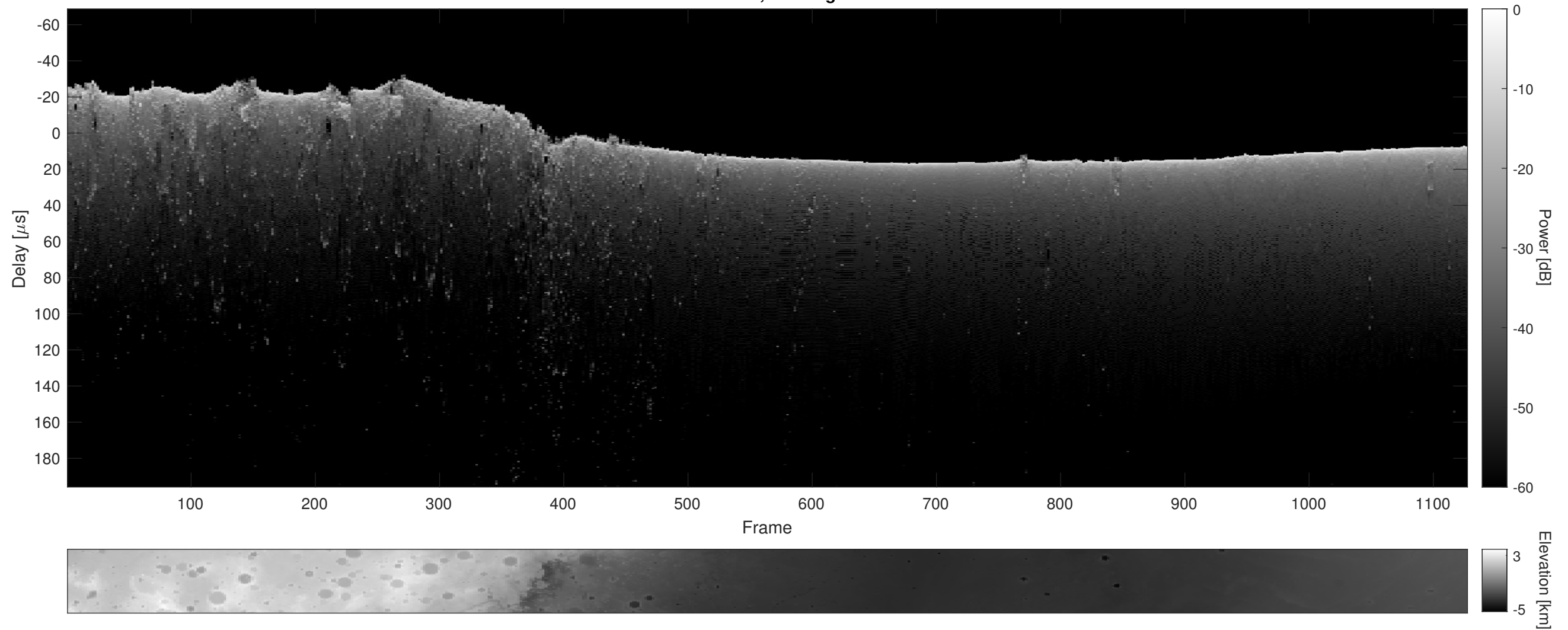
Orbit 14394, Cluttergram
