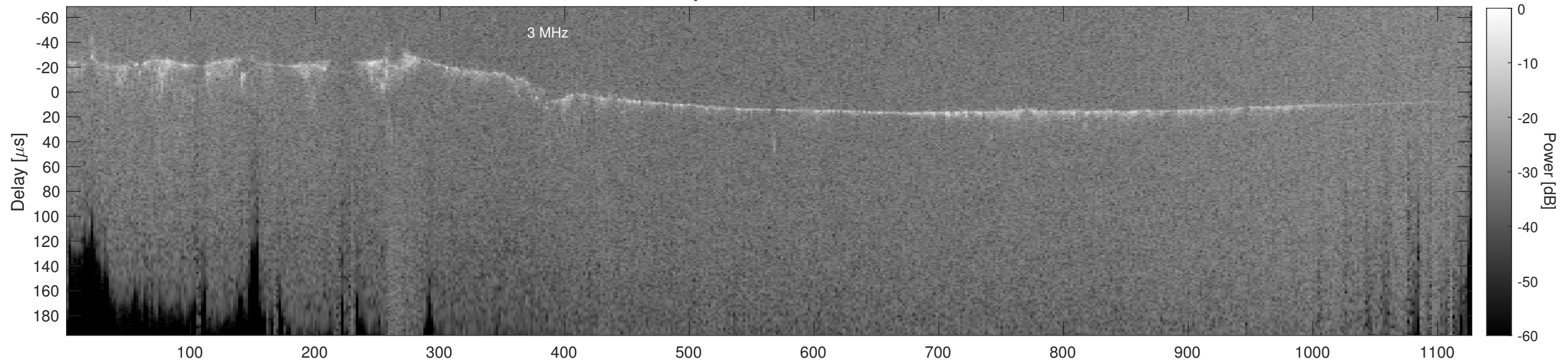
Orbit 14394, Cluttergram
