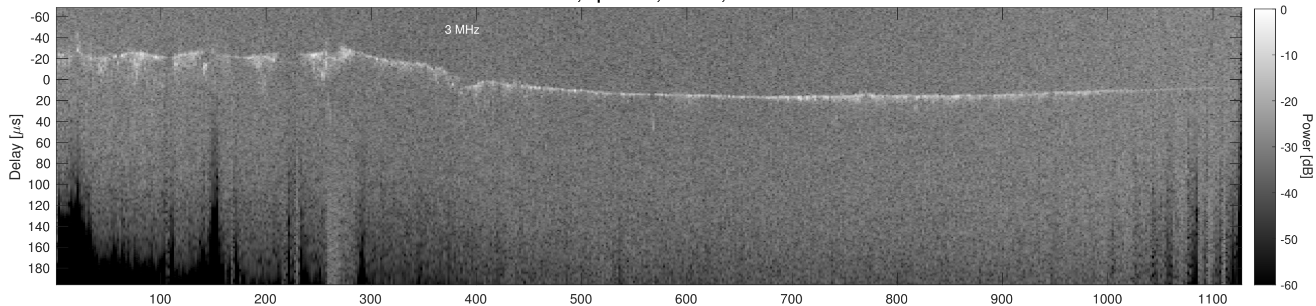
Orbit 14394, Cluttergram
