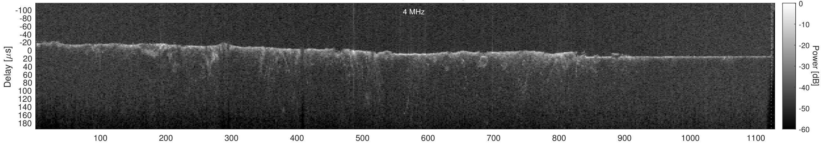
Orbit 14395, Cluttergram
