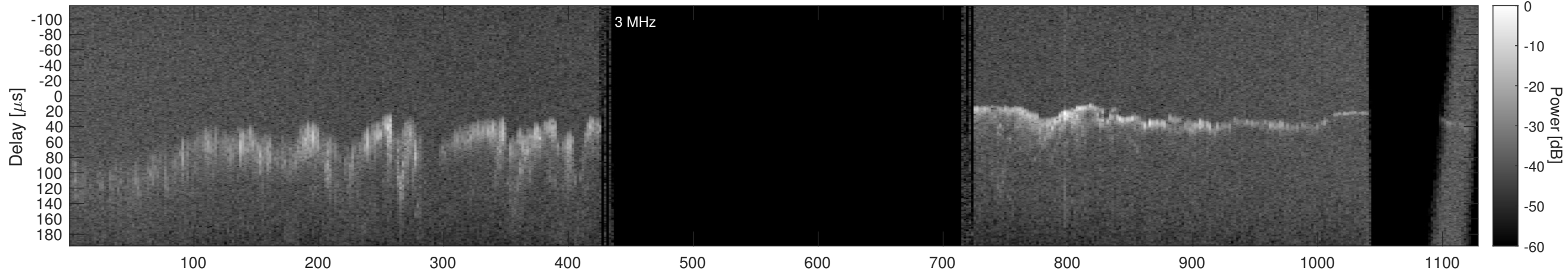
Orbit 14395, Window, Channel 2, Chapman
