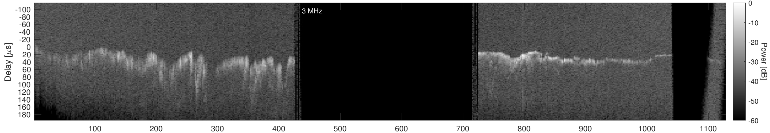
Orbit 14395, Window, Channel 2, Optimized
