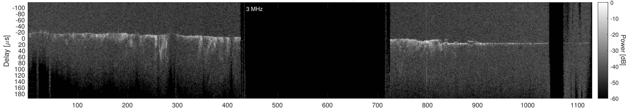
Orbit 14395, Cluttergram
