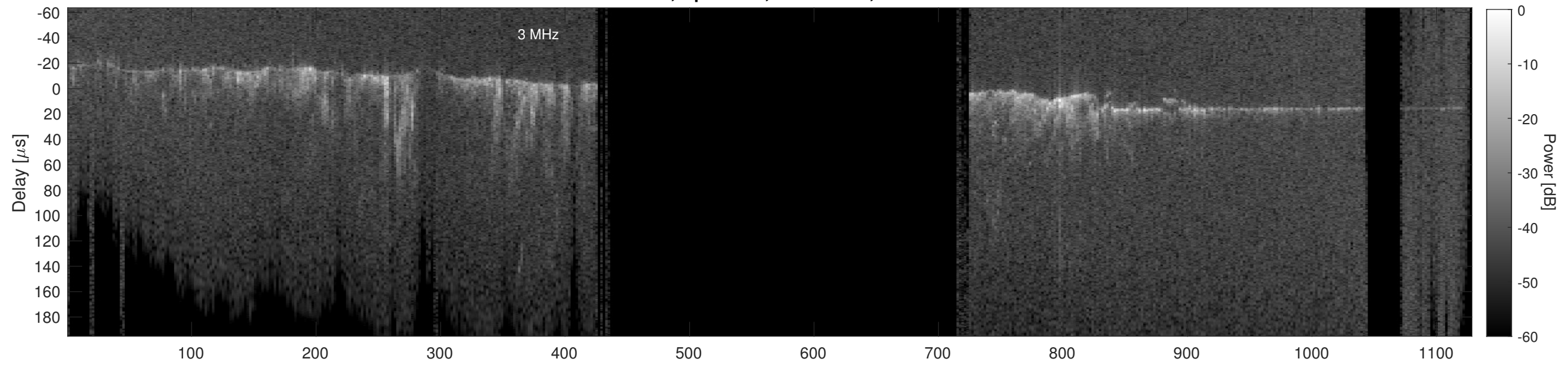
Orbit 14395, Cluttergram
