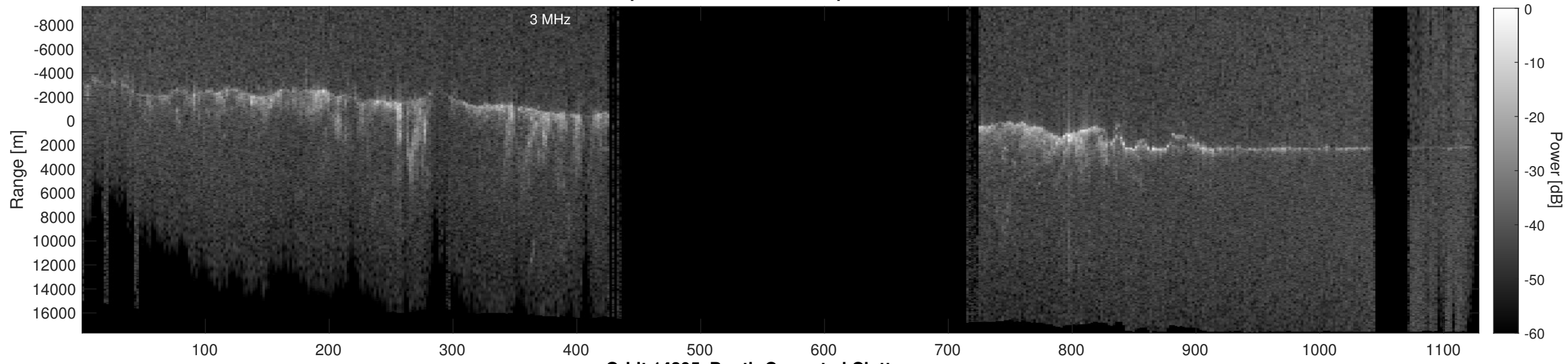
Orbit 14395, Depth-Corrected Cluttergram
