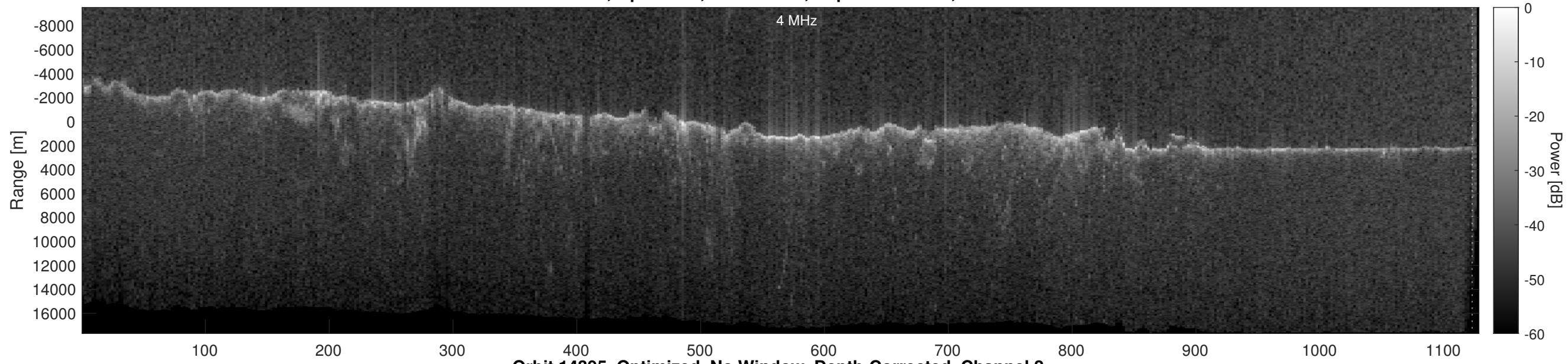
Orbit 14395, Optimized, No Window, Depth-Corrected, Channel 2
