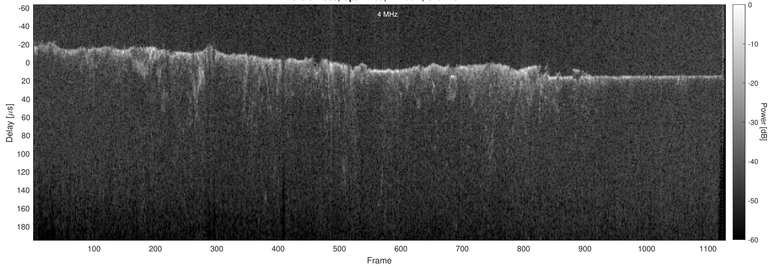
Orbit 14395, Optimized, Window, Channel 2
