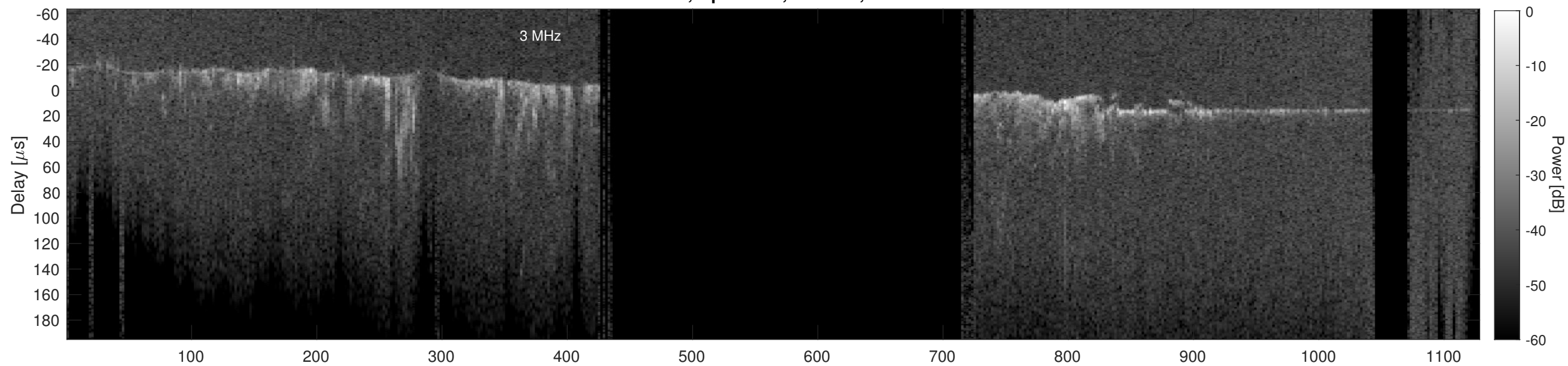
Orbit 14395, Cluttergram
