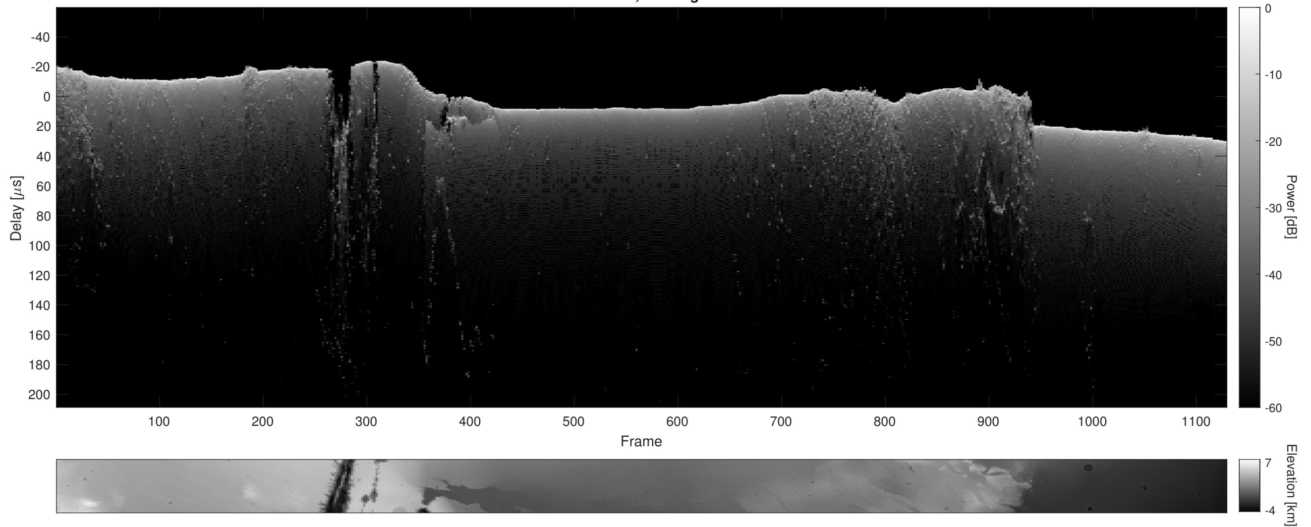
Orbit 14396, Cluttergram
