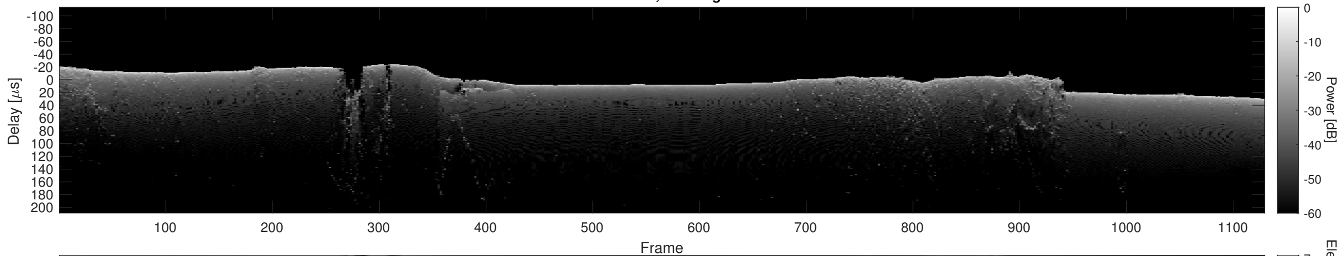
Orbit 14396, Cluttergram
