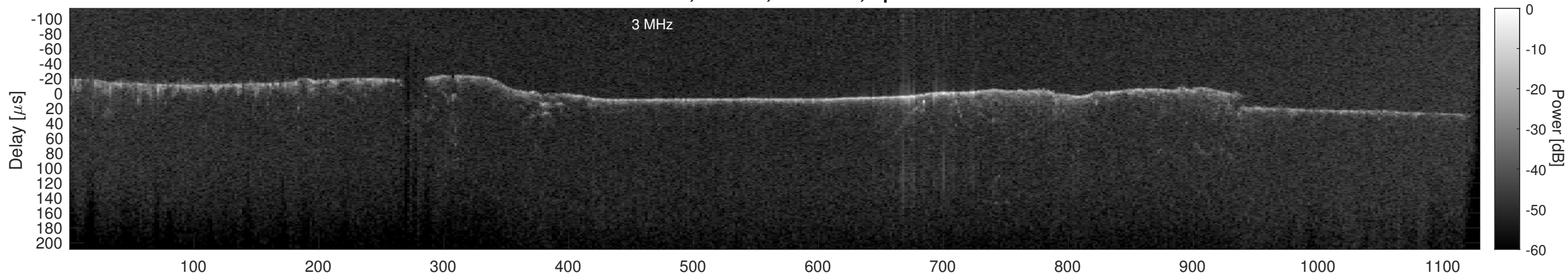
Orbit 14396, Cluttergram
