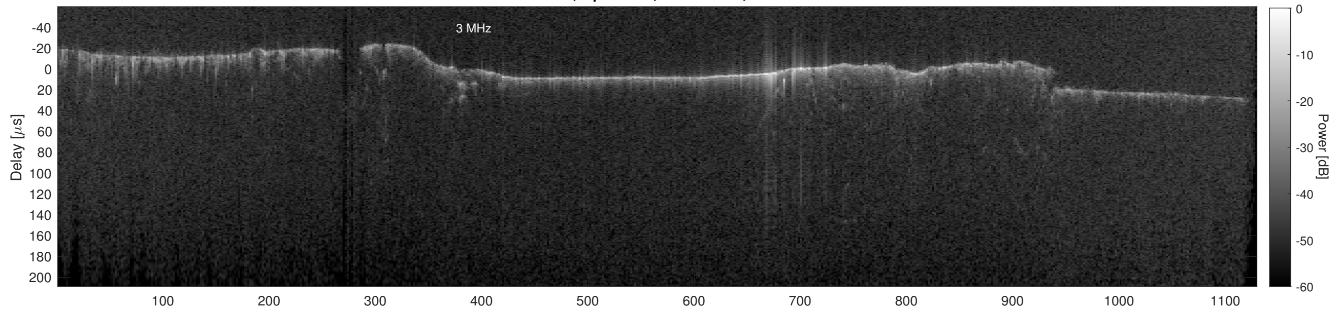
Orbit 14396, Cluttergram
