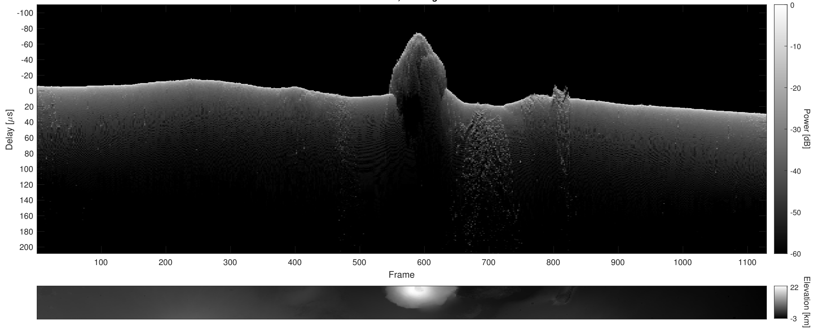
Orbit 14400, Cluttergram
