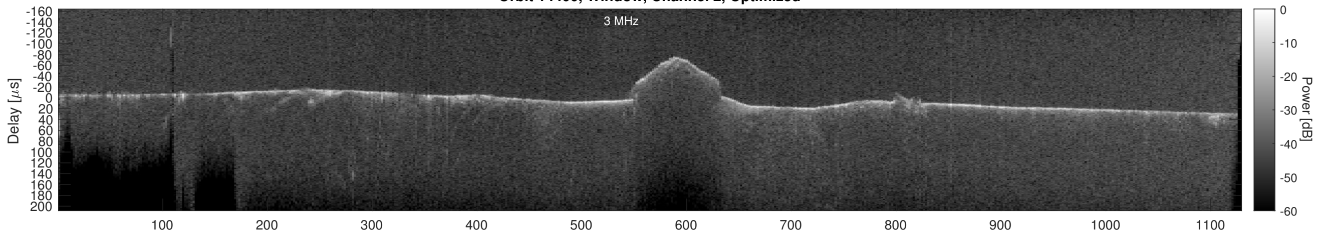
Orbit 14400, Cluttergram
