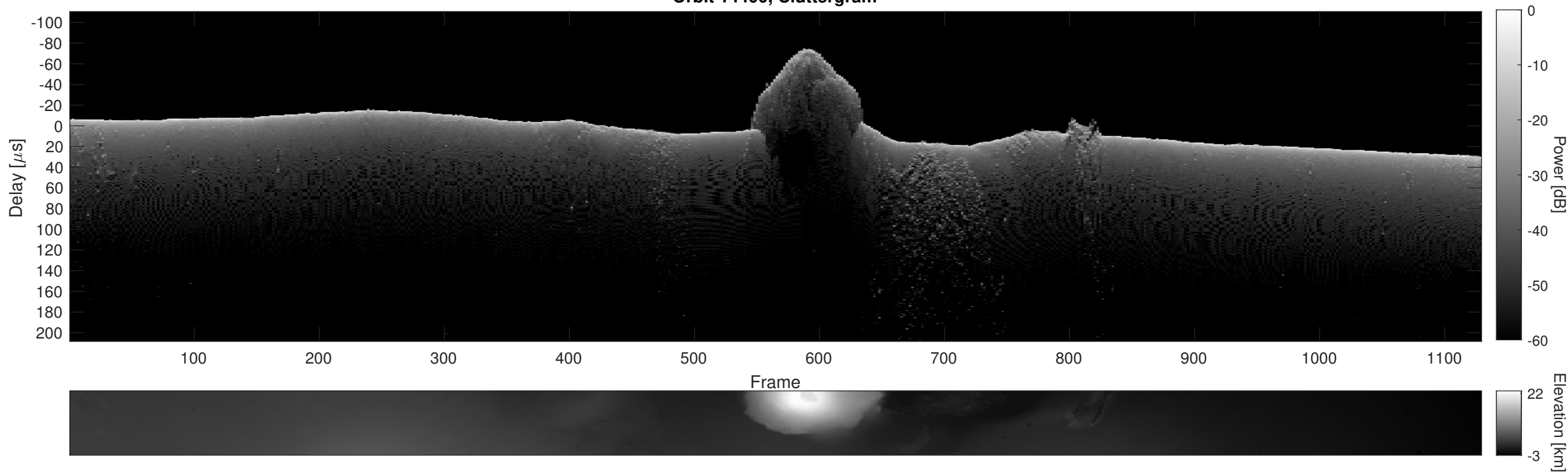
Orbit 14400, Cluttergram
