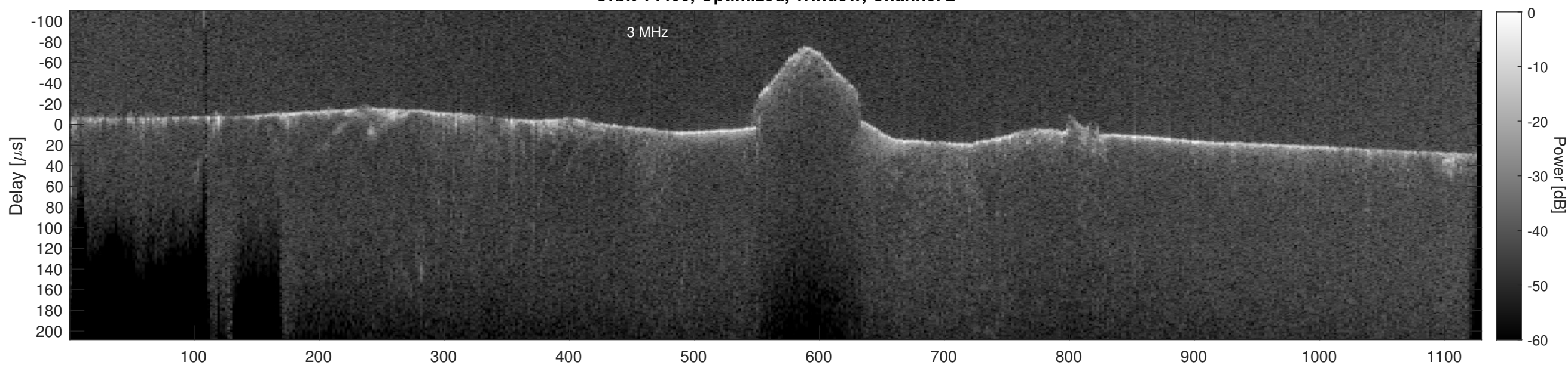
Orbit 14400, Cluttergram
