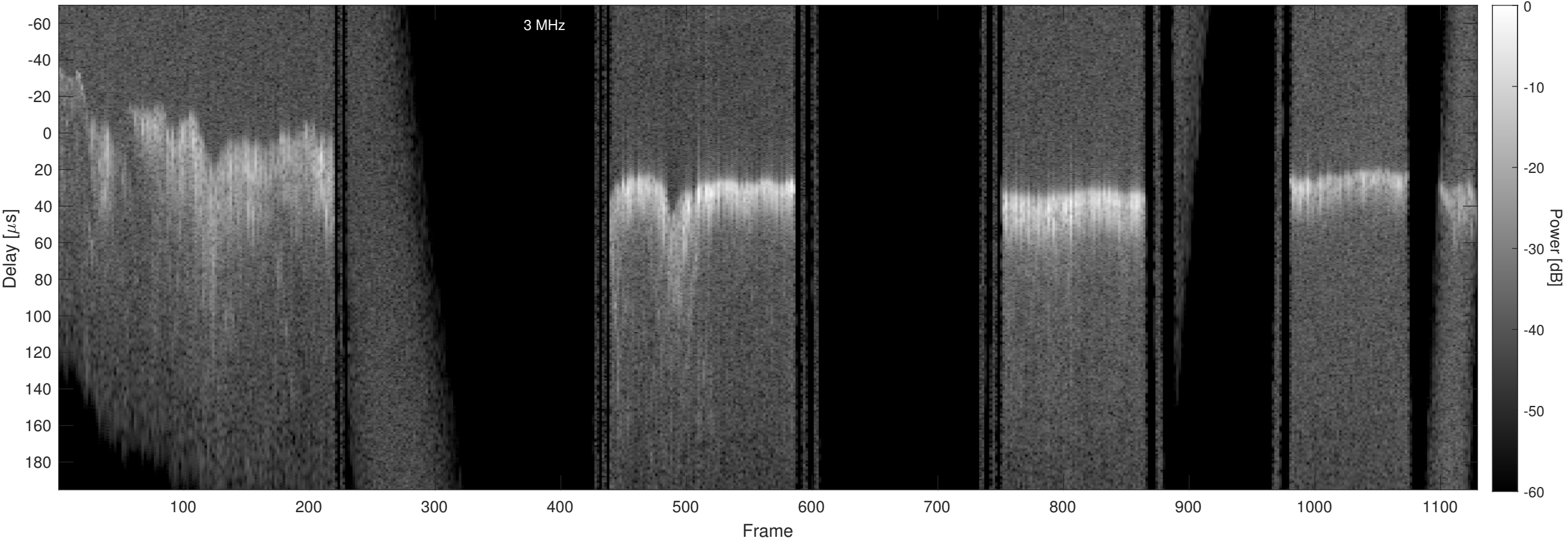
Orbit 14401, Chapman, No Window, Channel 2
