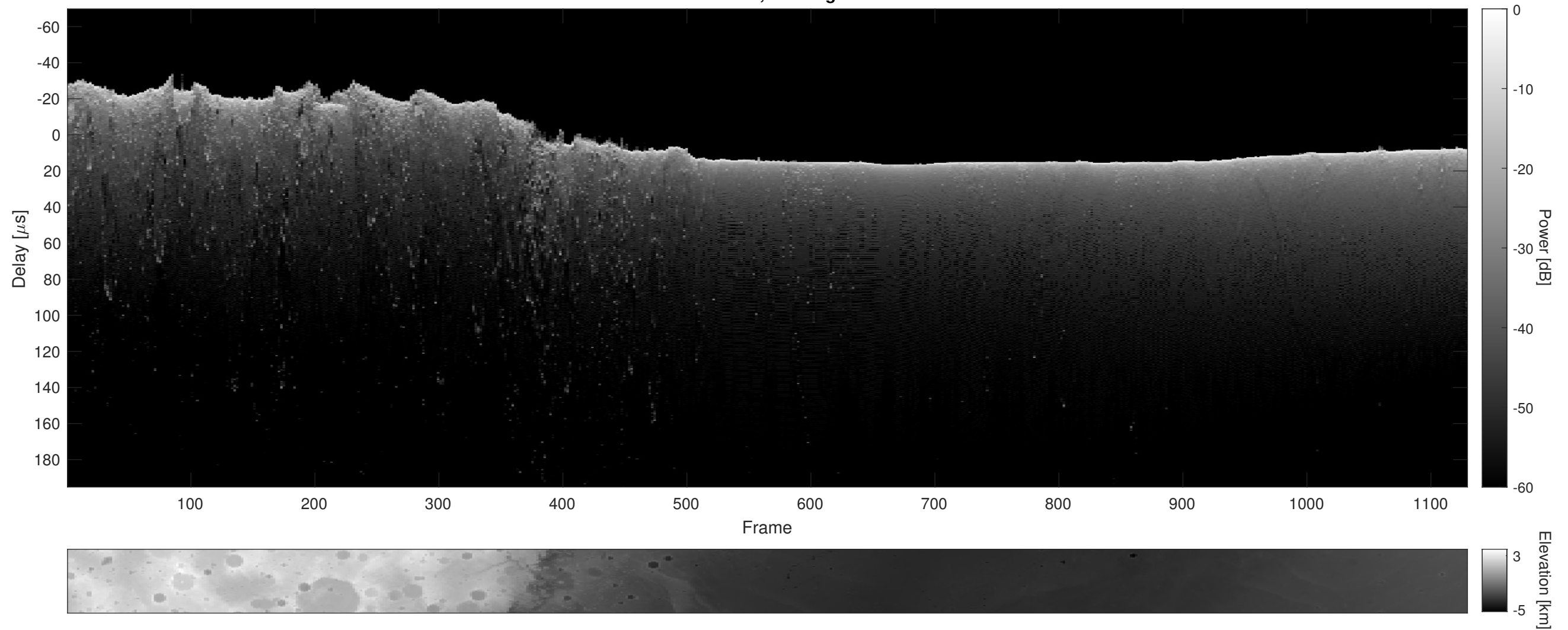
Orbit 14401, Cluttergram
