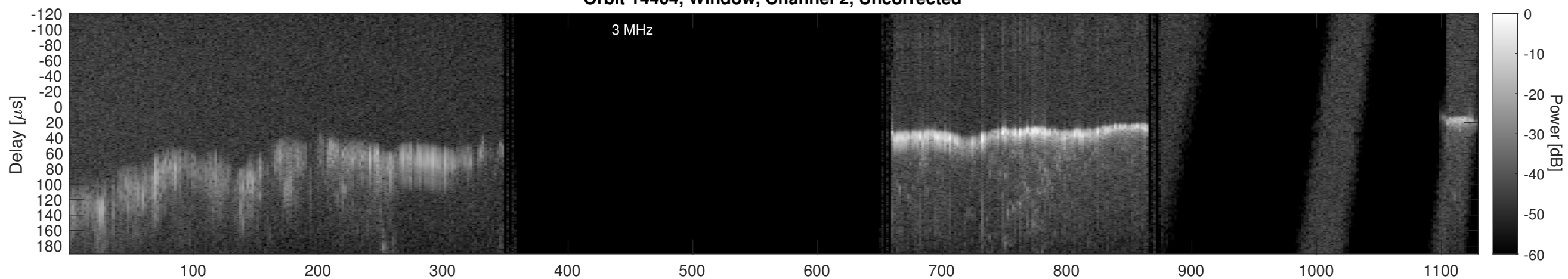
Orbit 14404, Window, Channel 2, Chapman
