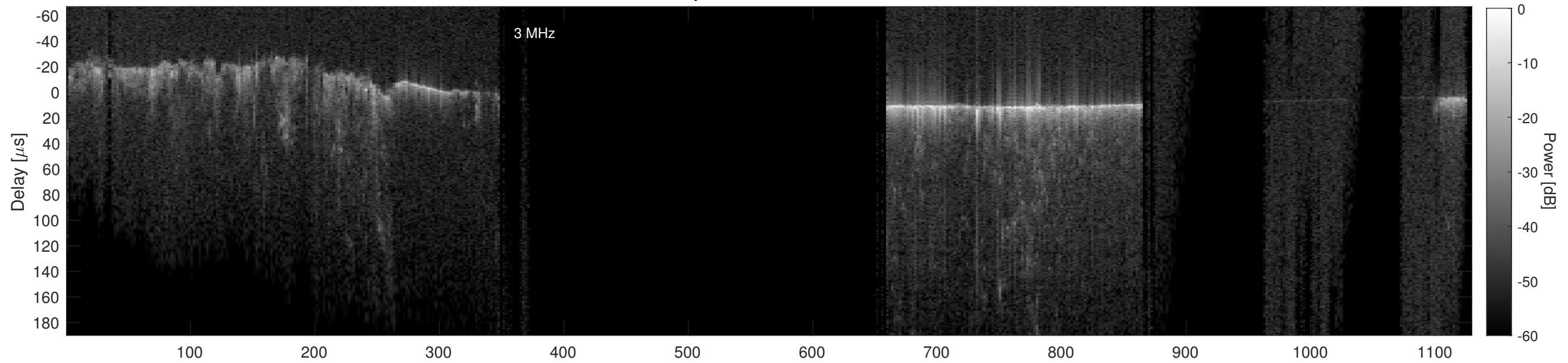
Orbit 14404, Cluttergram
