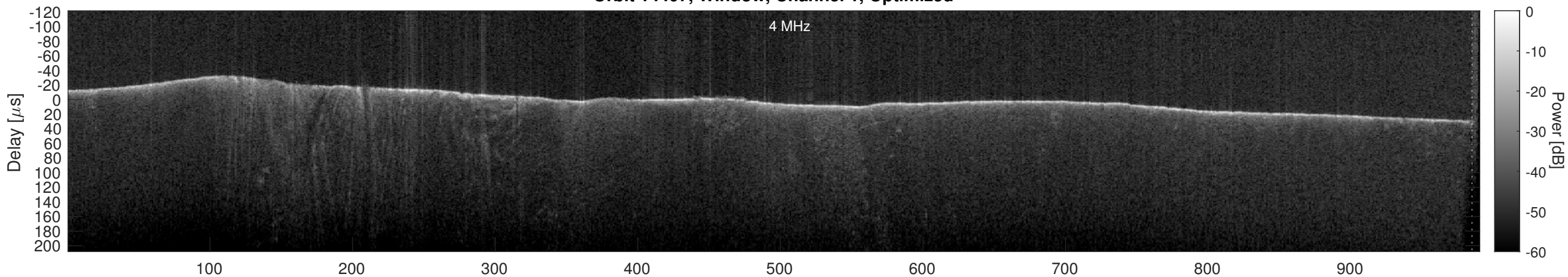
Orbit 14407, Cluttergram
