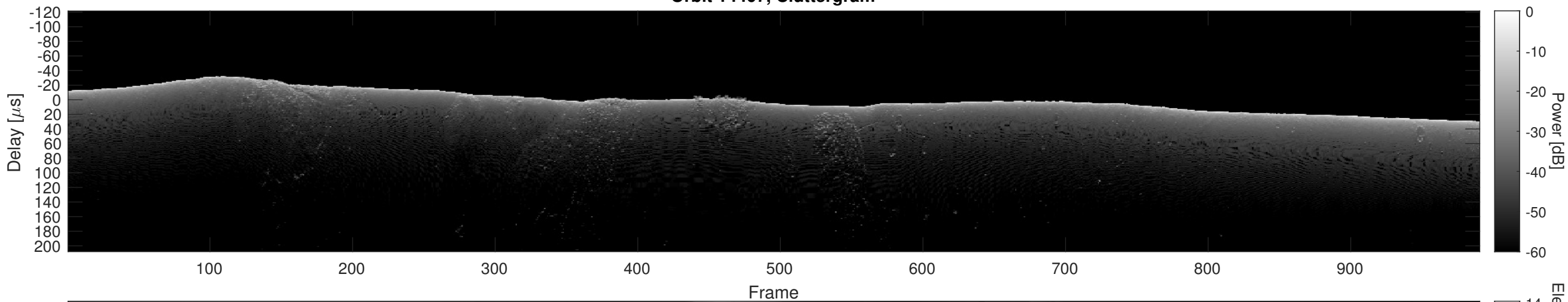
Orbit 14407, Cluttergram
