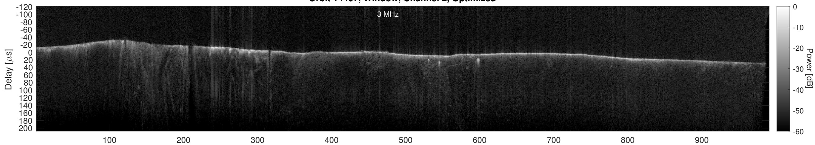
Orbit 14407, Cluttergram
