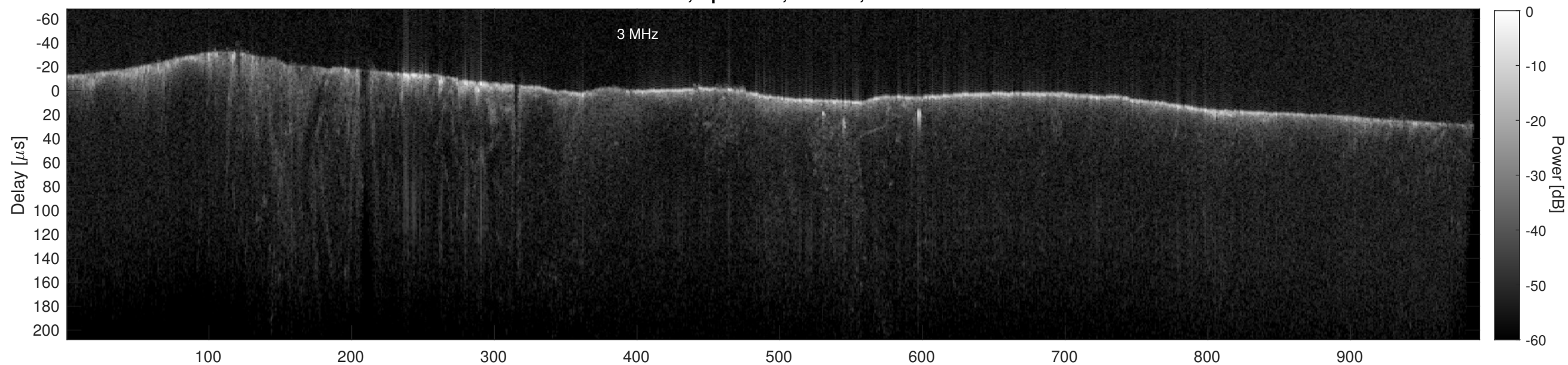
Orbit 14407, Cluttergram
