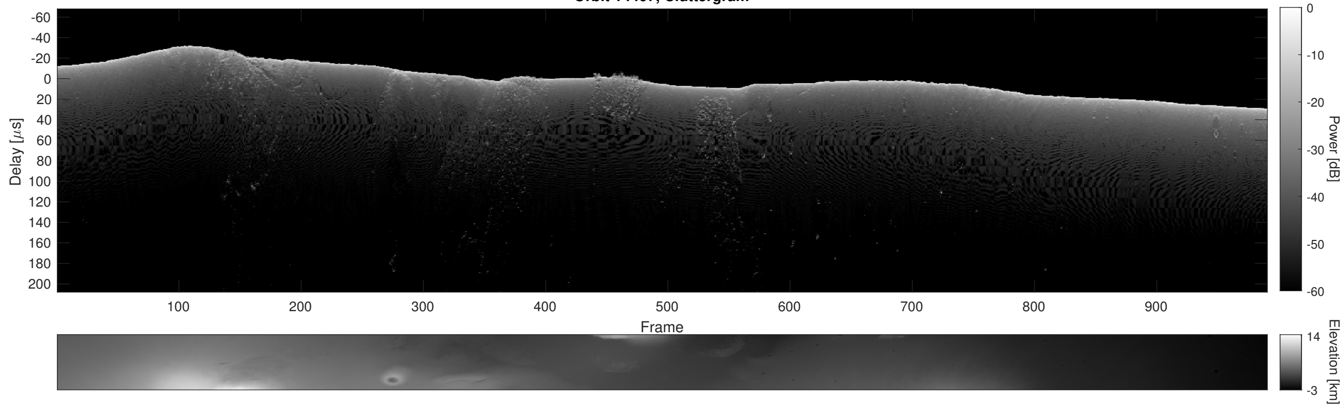
Orbit 14407, Cluttergram
