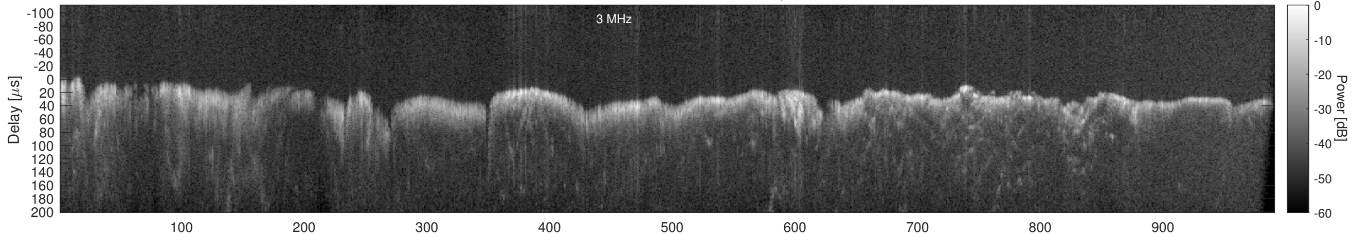
Orbit 14409, Window, Channel 2, Optimized
