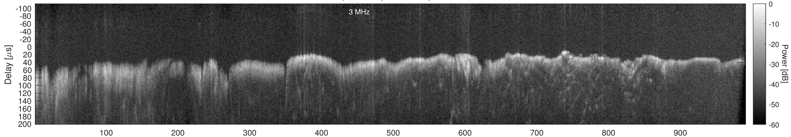
Orbit 14409, Window, Channel 2, Chapman
