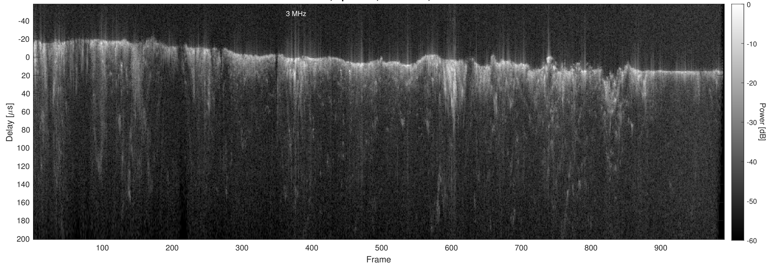
Orbit 14409, Optimized, No Window, Channel 2
