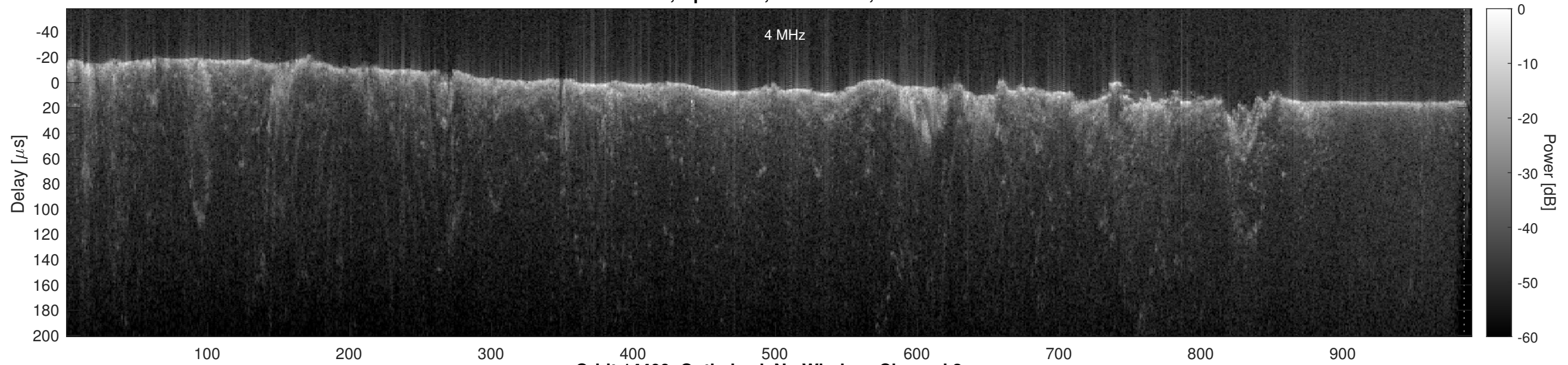
Orbit 14409, Optimized, No Window, Channel 2
