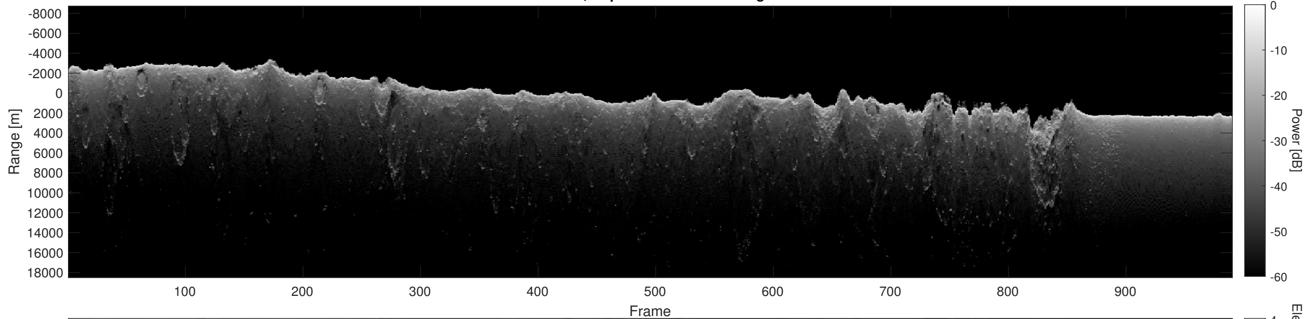
Orbit 14409, Depth-Corrected Cluttergram
