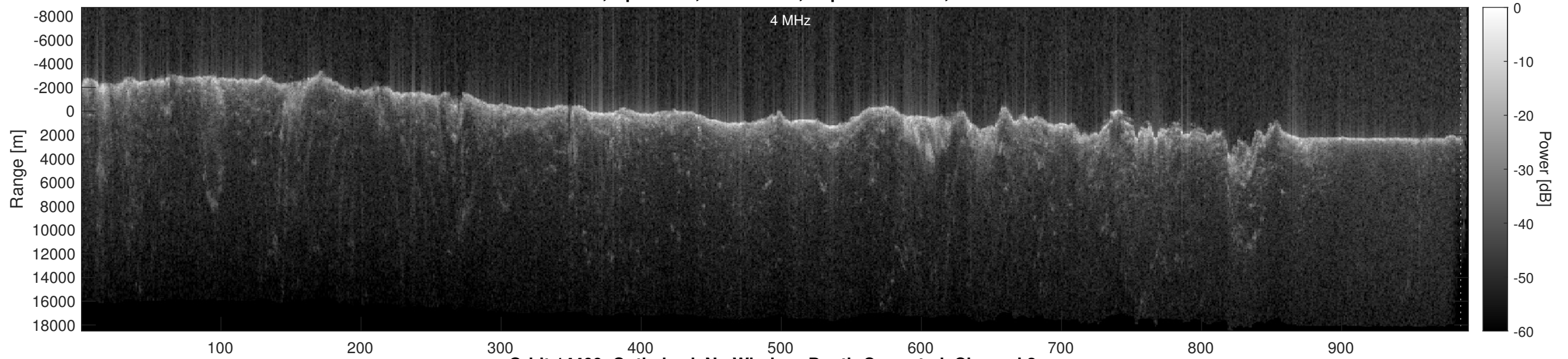
Orbit 14409, Optimized, No Window, Depth-Corrected, Channel 2
