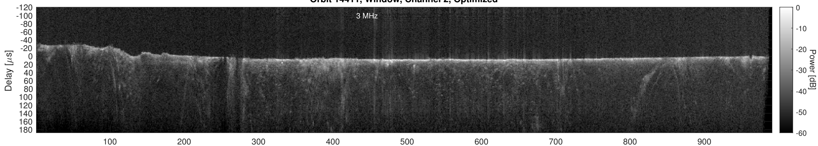
Orbit 14411, Cluttergram
