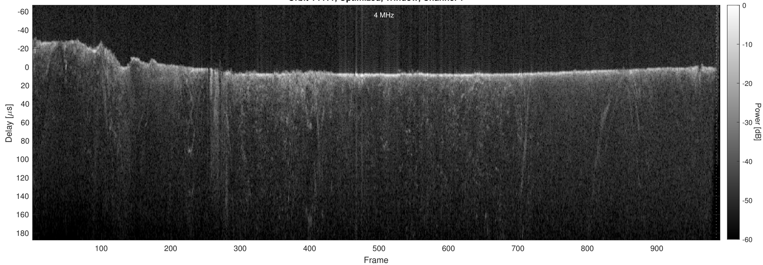
Orbit 14411, Optimized, Window, Channel 2
