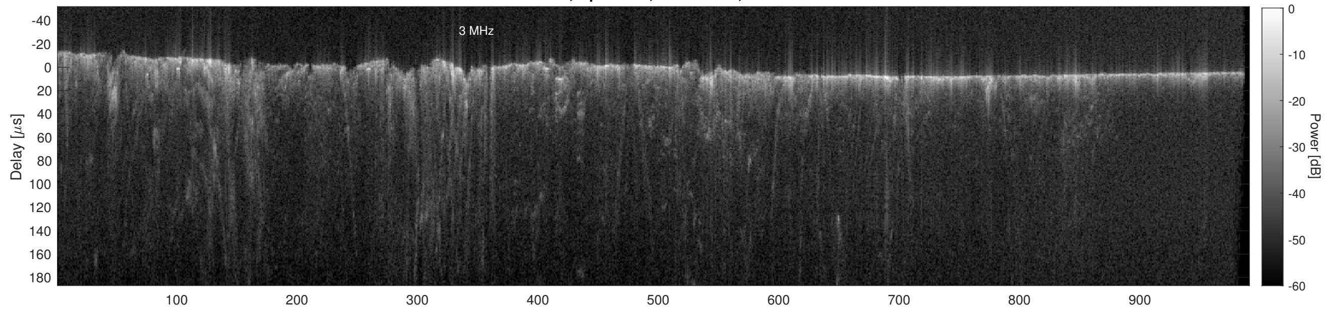
Orbit 14413, Cluttergram
