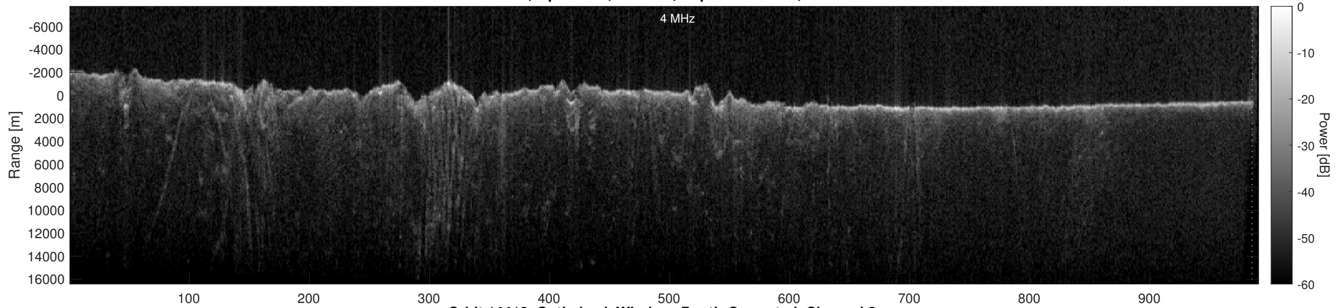
Orbit 14413, Optimized, Window, Depth-Corrected, Channel 2
