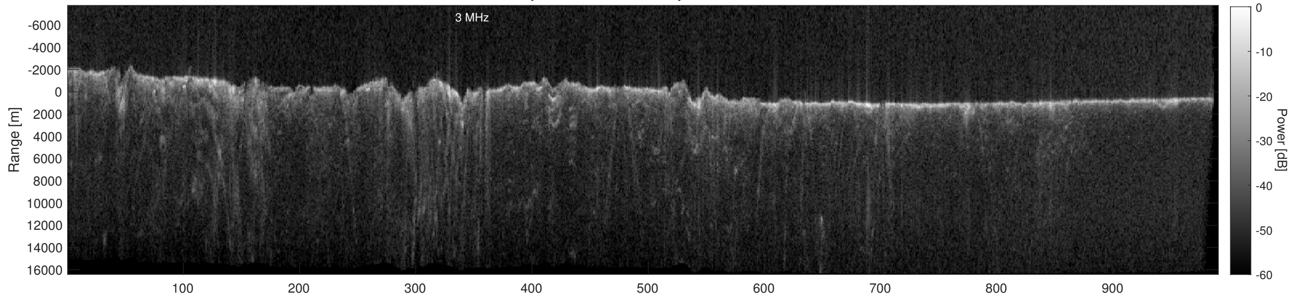
Orbit 14413, Depth-Corrected Cluttergram
