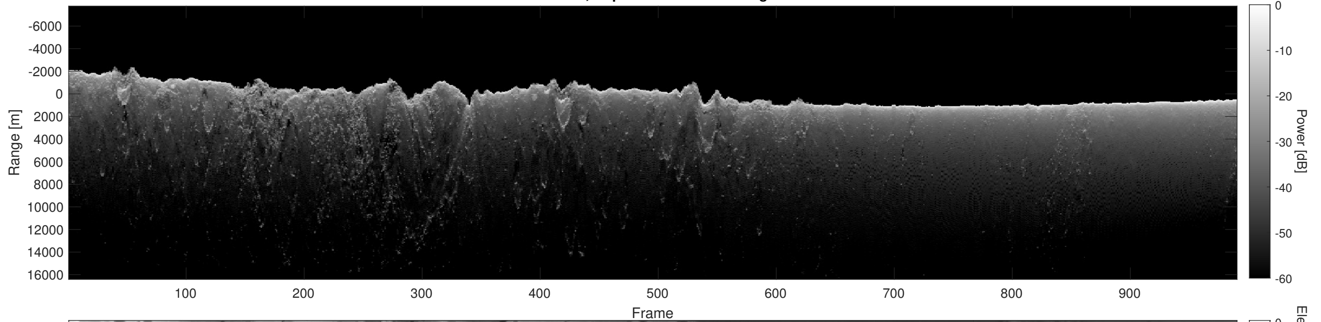
Orbit 14413, Depth-Corrected Cluttergram
