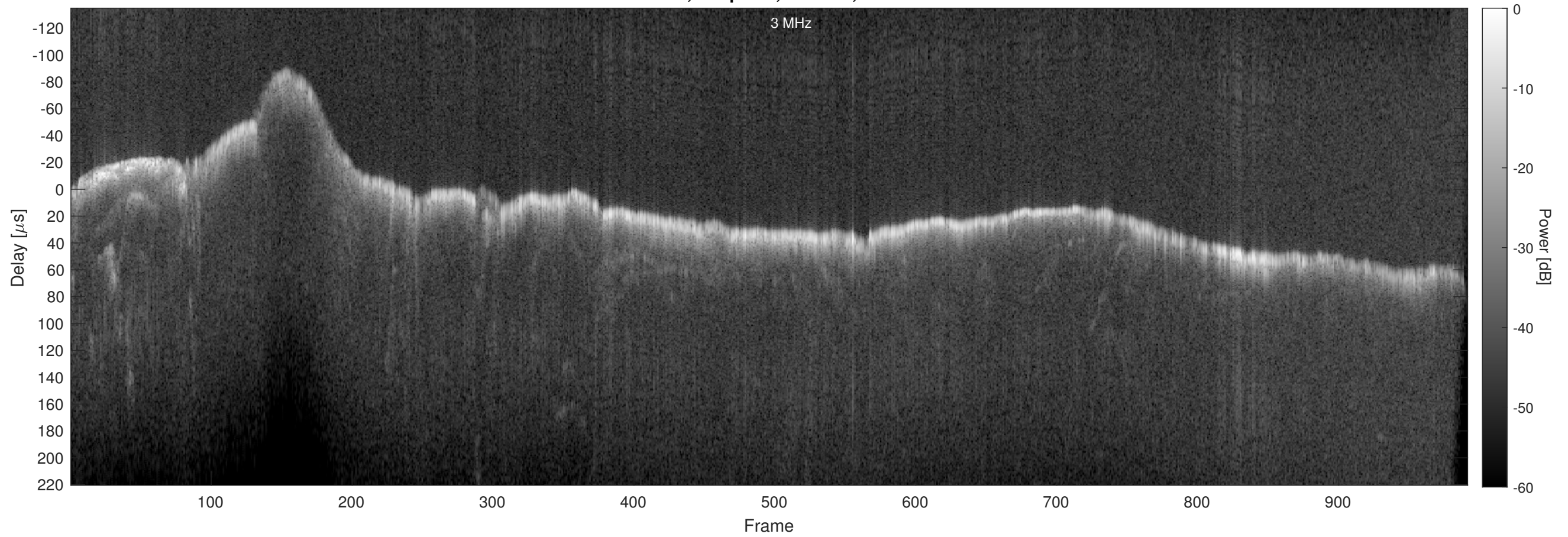
Orbit 14414, Chapman, Window, Channel 2
