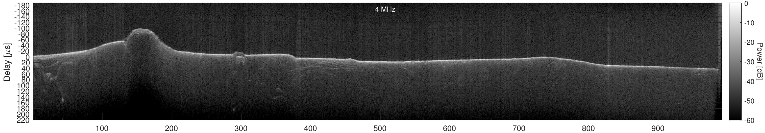
Orbit 14414, Cluttergram
