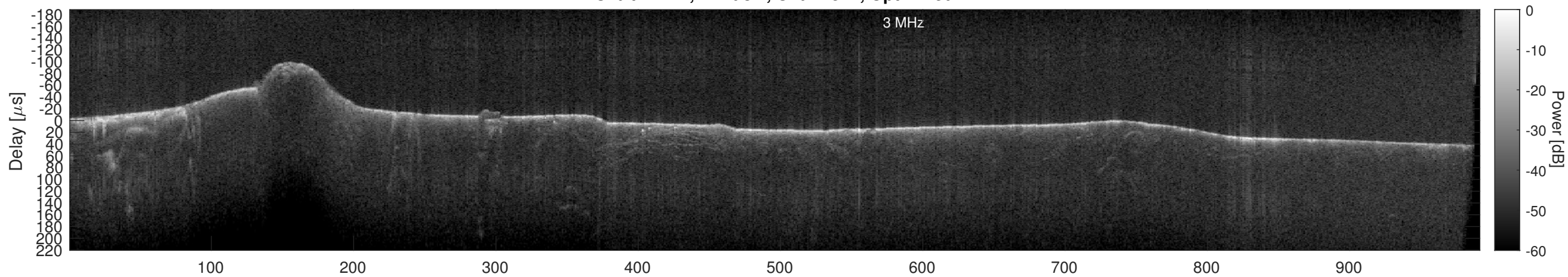
Orbit 14414, Cluttergram
