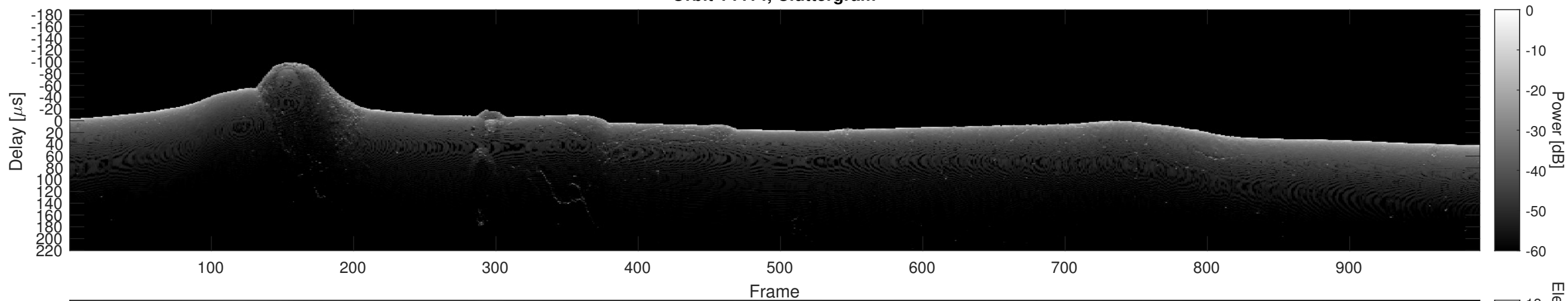
Orbit 14414, Cluttergram
