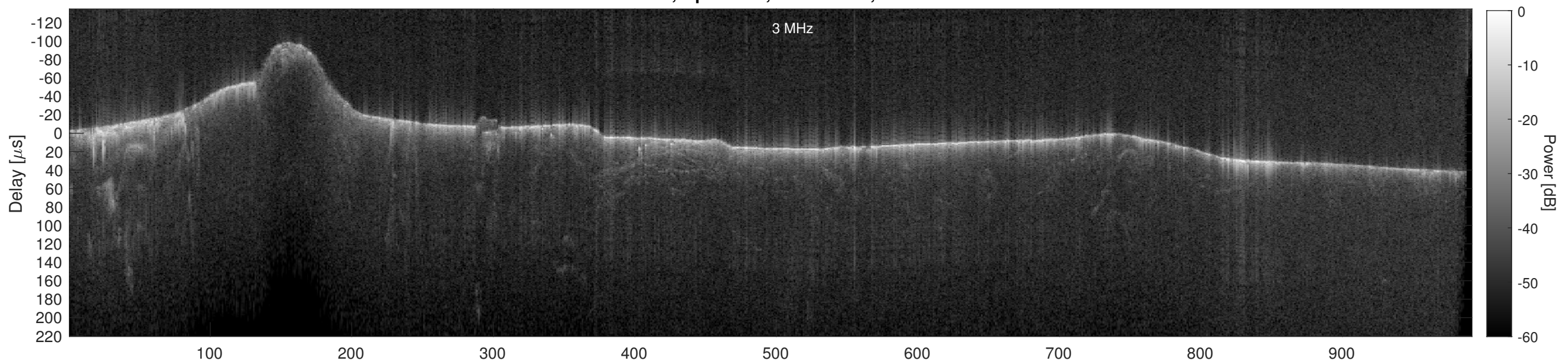
Orbit 14414, Cluttergram
