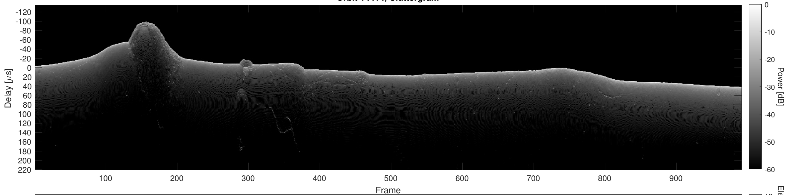
Orbit 14414, Cluttergram
