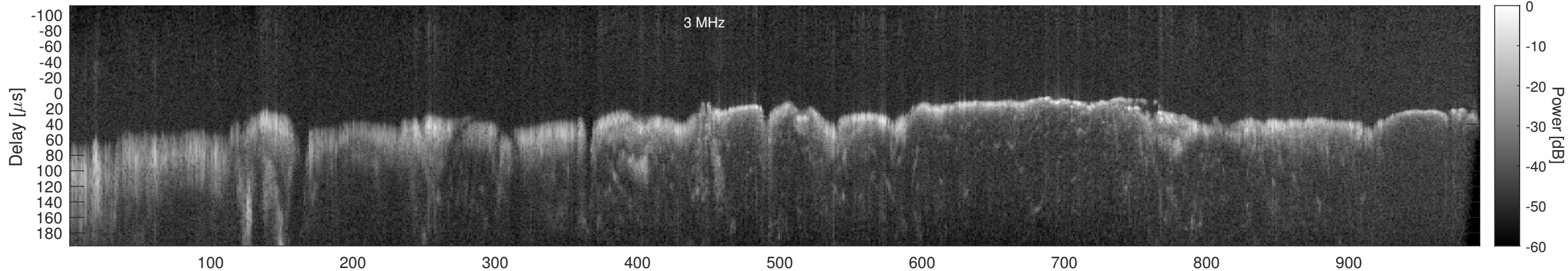
Orbit 14416, Window, Channel 2, Chapman
