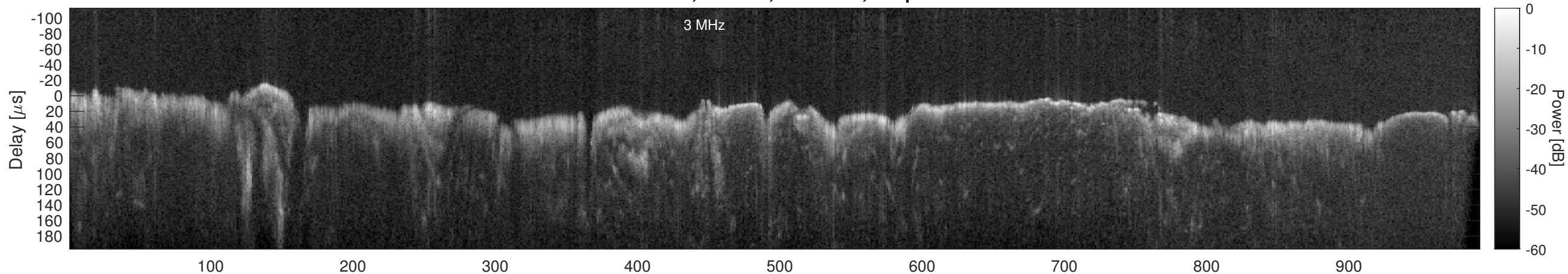
Orbit 14416, Window, Channel 2, Optimized
