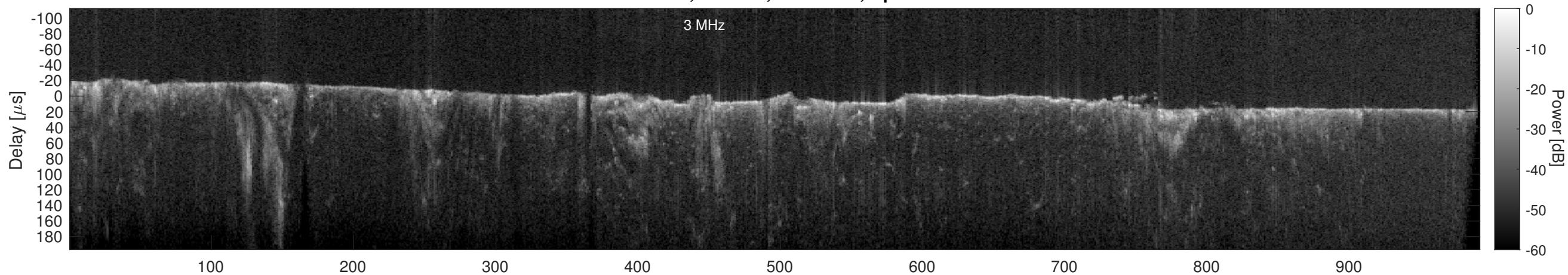
Orbit 14416, Cluttergram
