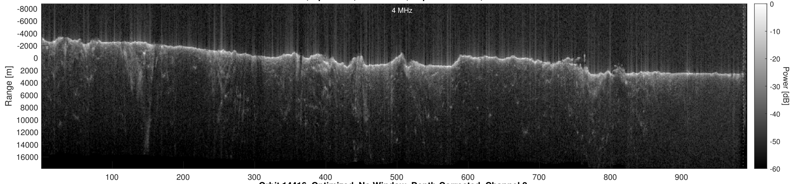
Orbit 14416, Optimized, No Window, Depth-Corrected, Channel 2
