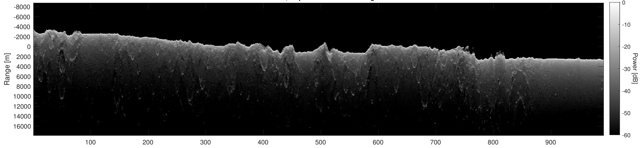
Orbit 14416, Depth-Corrected Cluttergram
