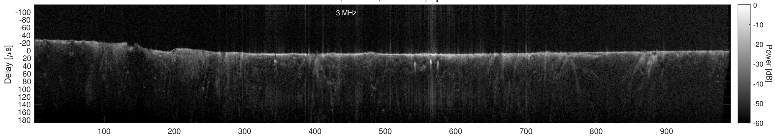
Orbit 14418, Cluttergram
