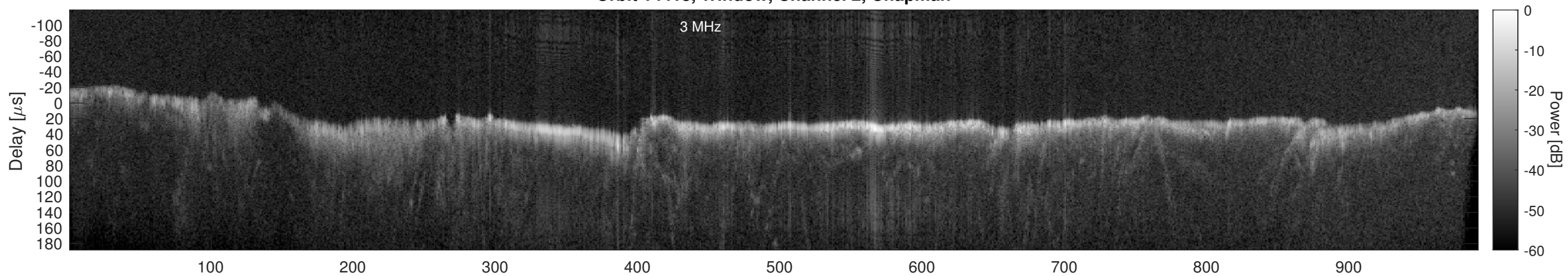
Orbit 14418, Window, Channel 2, Optimized
