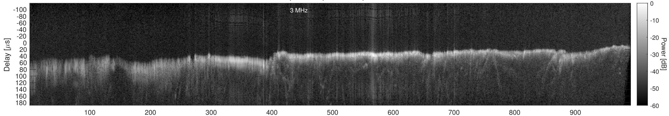
Orbit 14418, Window, Channel 2, Chapman
