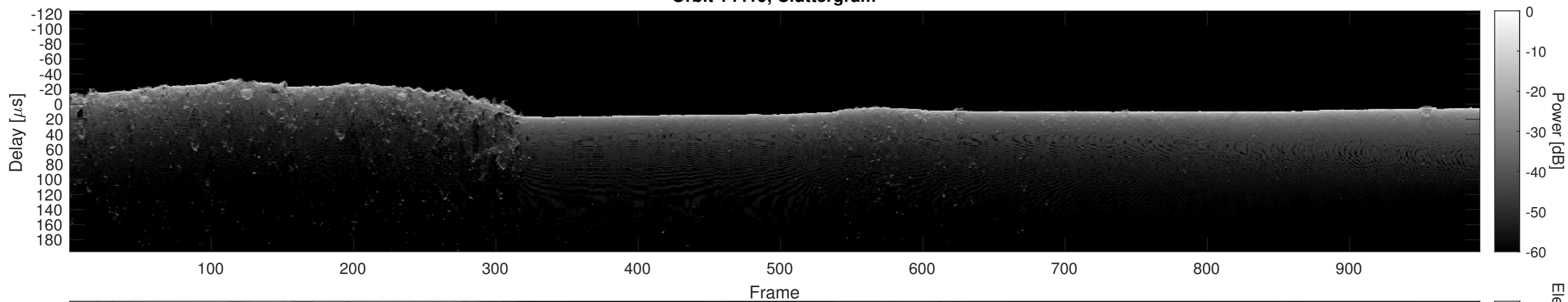
Orbit 14419, Cluttergram
