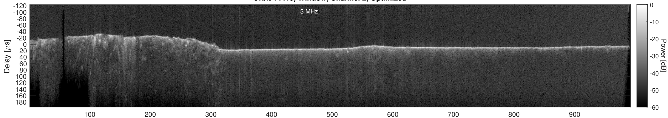
Orbit 14419, Cluttergram
