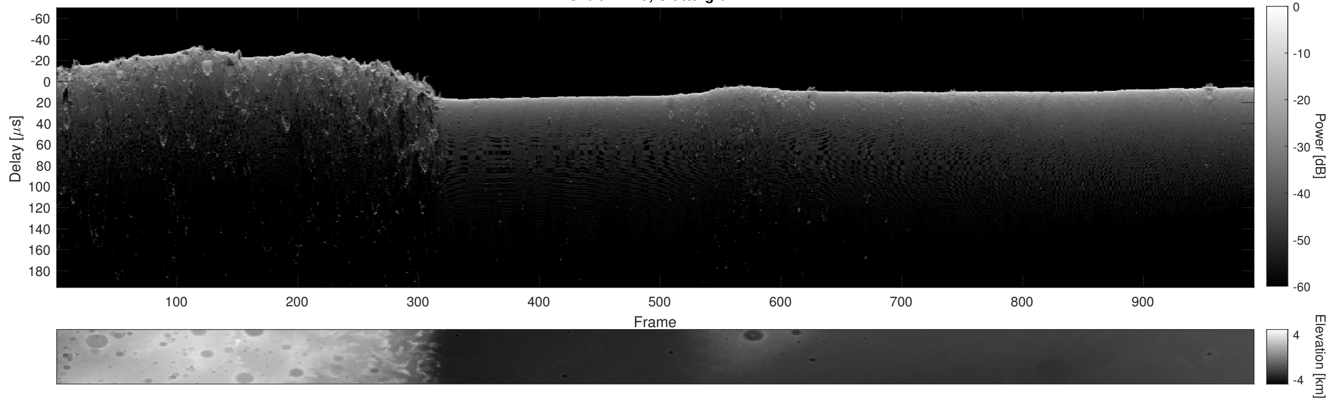
Orbit 14419, Cluttergram
