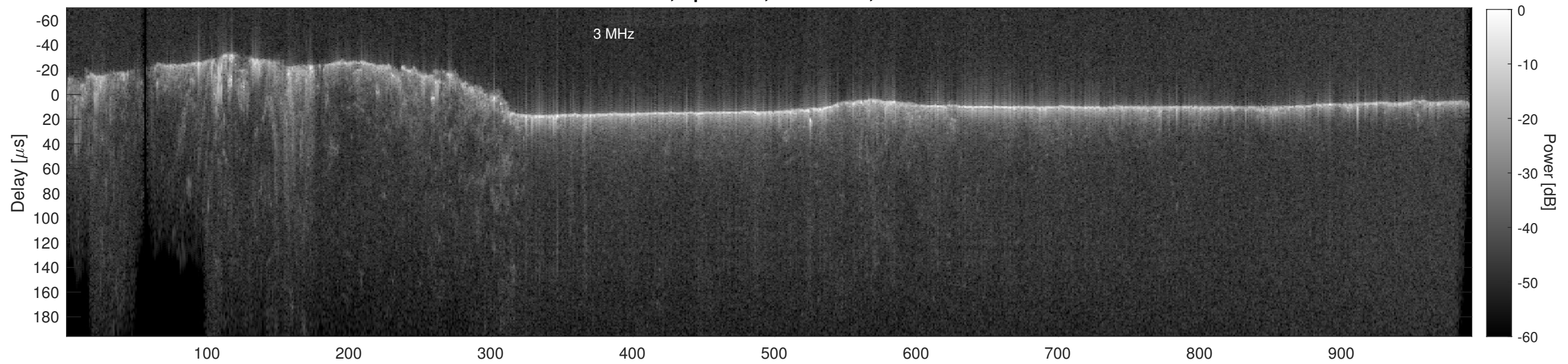
Orbit 14419, Cluttergram
