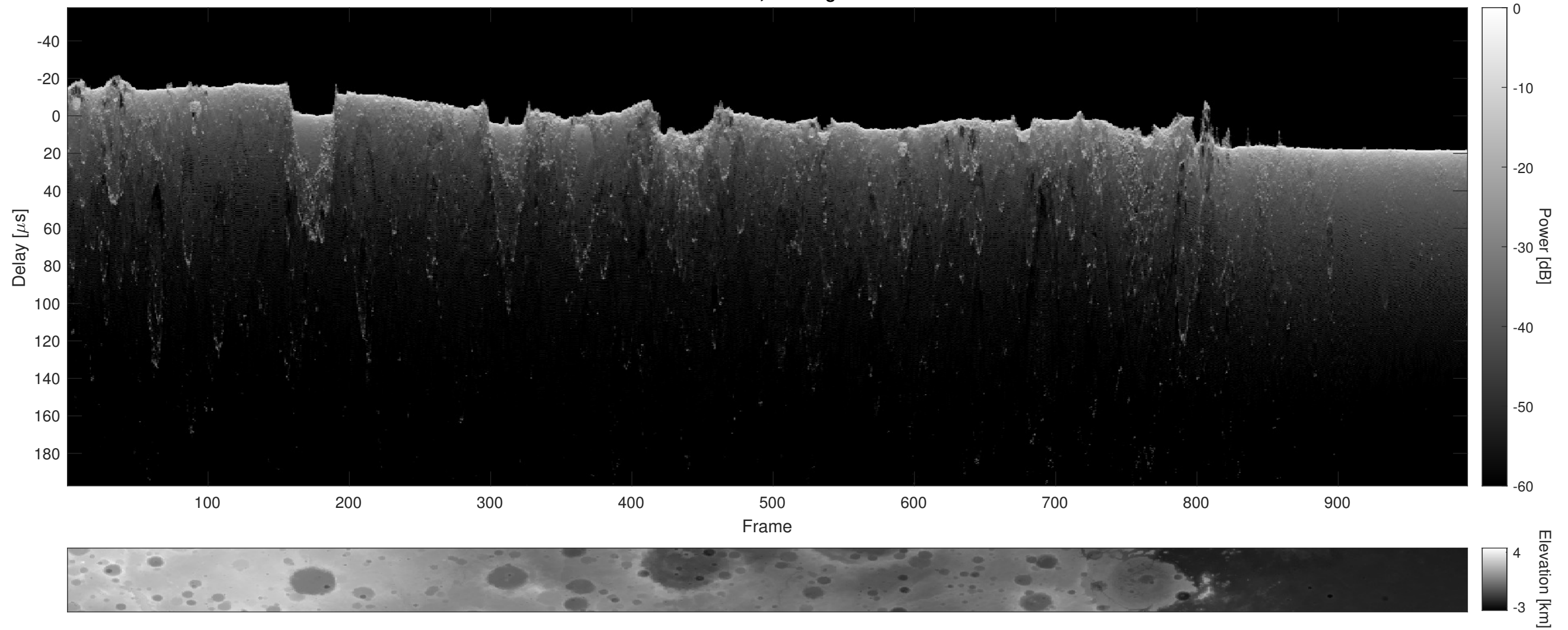
Orbit 14423, Cluttergram
