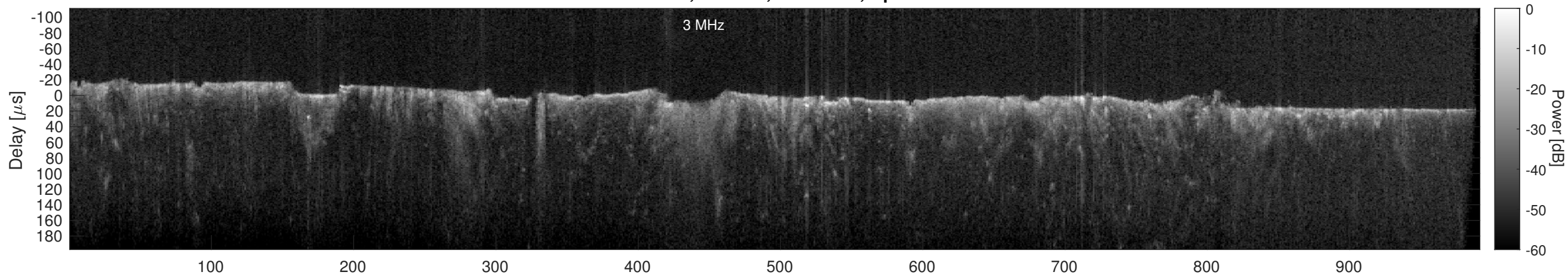
Orbit 14423, Cluttergram
