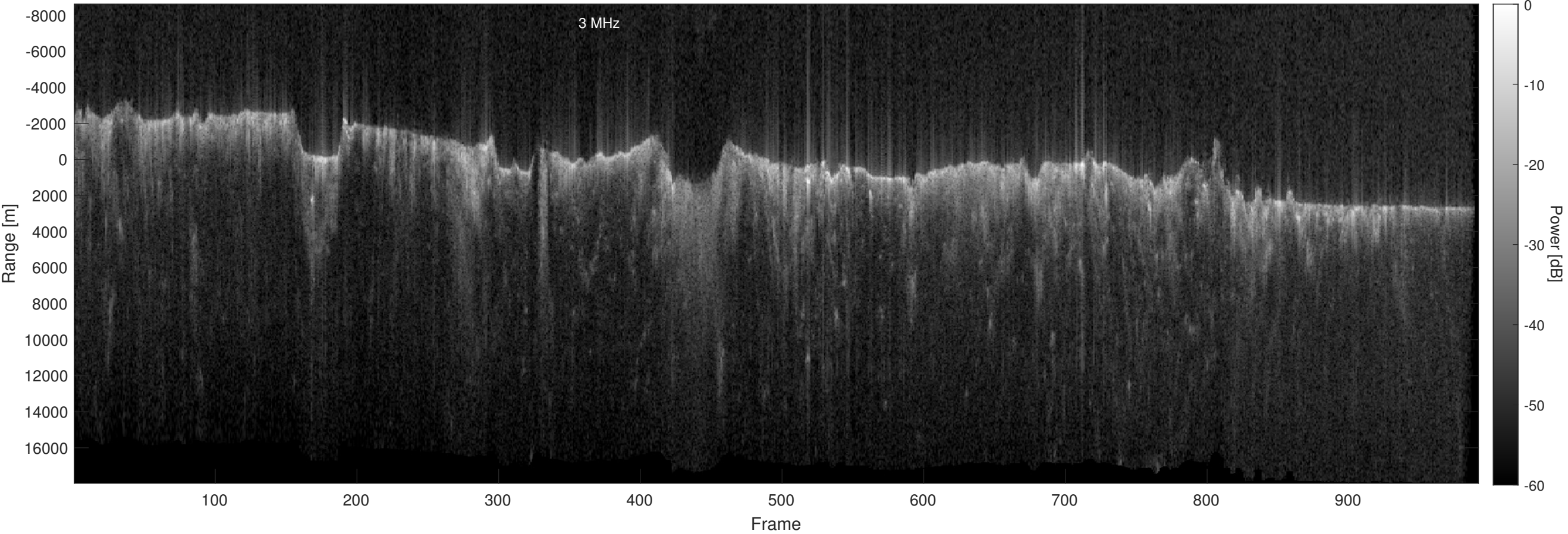
Orbit 14423, Optimized, No Window, Depth-Corrected, Channel 2
