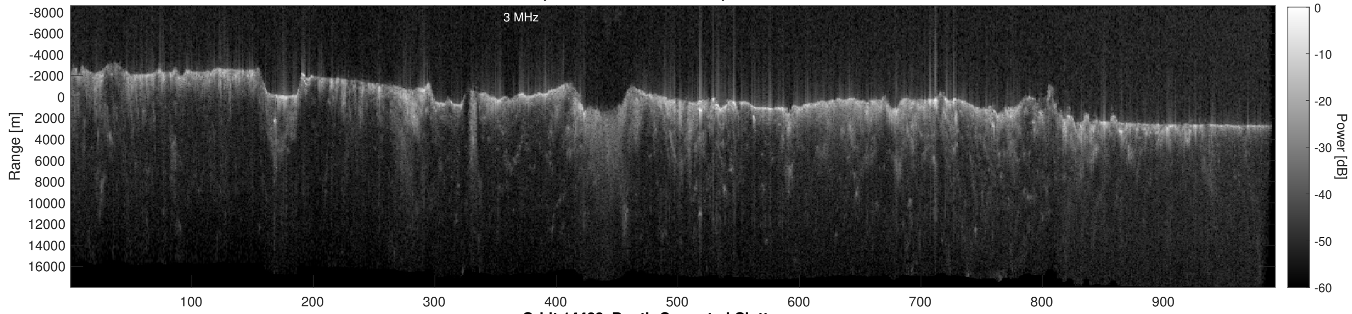
Orbit 14423, Depth-Corrected Cluttergram
